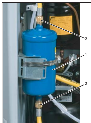
Fig. 31: Replacing filter
