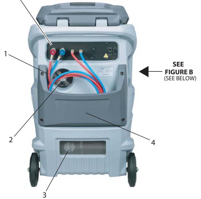
Fig. 2: Rear View
